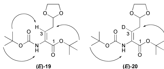
Fig. 2 Observed ^1\text{H} NMR nOes for ( E )- 19 and ( E )- 20 .
