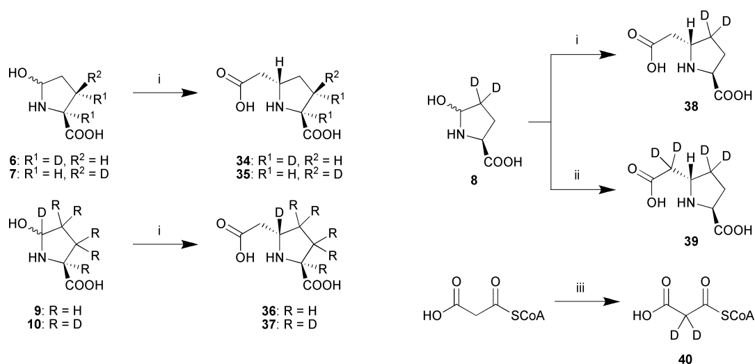
Scheme 5 Preparation of deuterated t -CMP derivatives 34–39 using CarB and/or ThnE ( D = {}^2H ). Reagents and conditions : (i) solution of L-GSA derivative from deprotection reaction, malonyl-CoA, CarB or ThnE (for 37 and 38 ), tris-HCl buffer (pH 9.0), 37 °C, 10 min; (ii) solution of 8 from deprotection reaction, [ {}^2H_2 ]-malonyl-CoA 40 , CarB, [ {}^2H_{11} ]-tris- {}^2H Cl buffer in {}^2H_2O (p {}^2H 9.0, uncorrected), 37 °C, 10 min; (iii) [ {}^2H_{11} ]-tris- {}^2H Cl buffer in {}^2H_2O (p {}^2H 7.5, uncorrected), 37 °C, 18 h.
