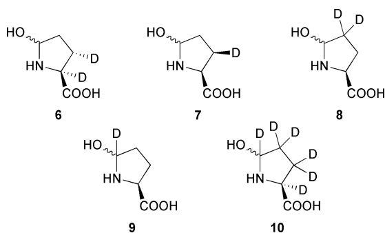
Fig. 1 Target compounds 6–10 ( \text{D} = ^2\text{H} ).
